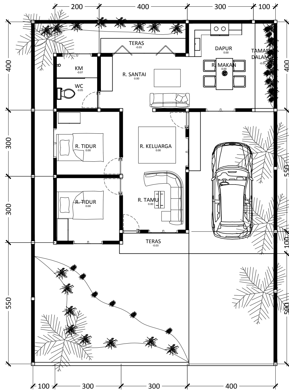
DENAH skala 1:100
